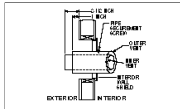
Figure 8 Venting Through the Wall
