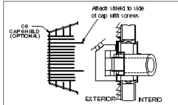
Figure 10A Termination Cap
