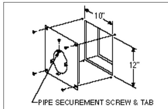
Figure 7 Interior Wall Shield
