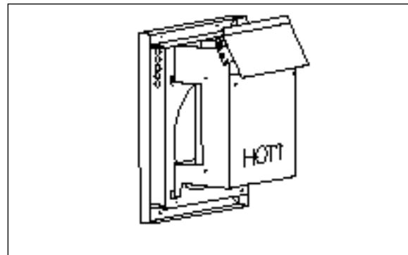
Figure 10B Proper Positioning of Termination Cap & Shield
