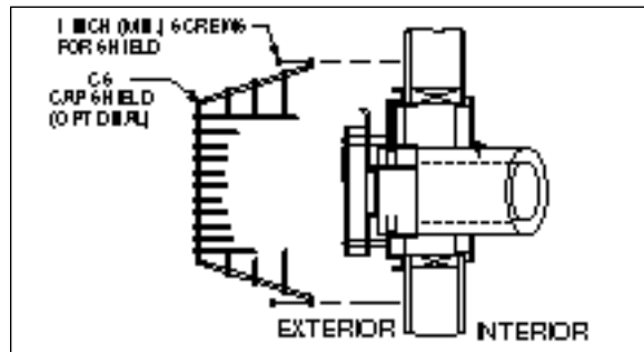
Figure 11 Cap Shield
