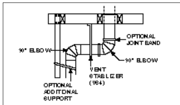
Figure 12 Elbows with stabilizer
