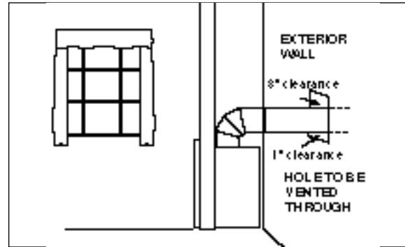
Figure 6 Exterior Wall Hole
