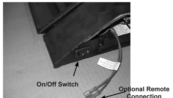
Figure 3A Control Box for IPI
