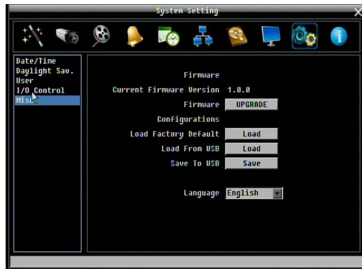
Figure 4-37 System Menu – Firmware & Misc.
