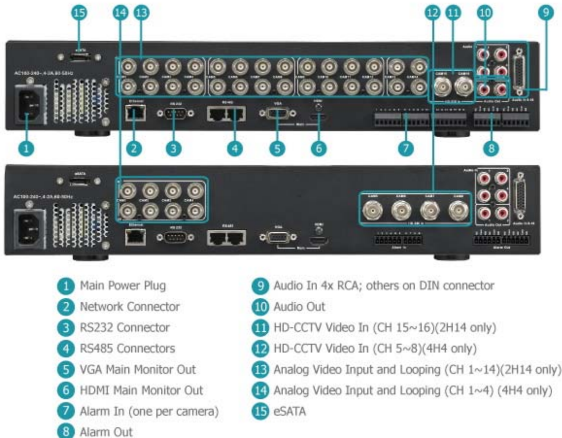
Figure 1-2 Rear Panel
