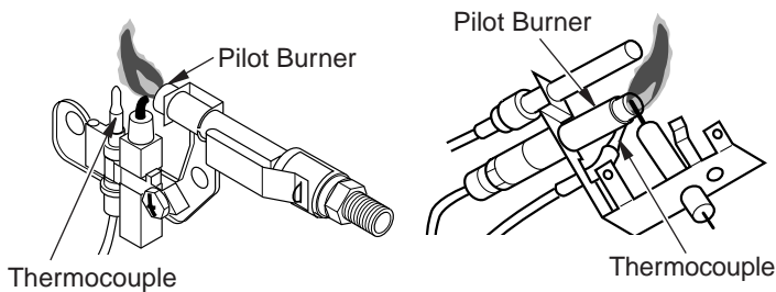
Figure 17 - Incorrect Pilot Flame Pattern (Your pilot may vary from pilots shown)
