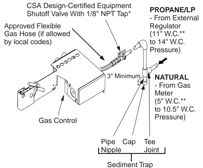
Figure 9 - Gas Connection
