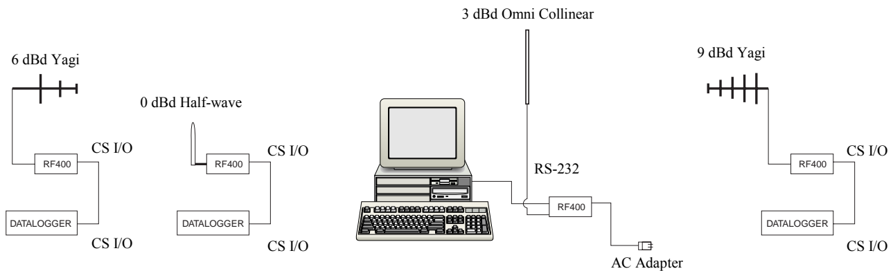
FIGURE 8. Point-to-Multipoint System
