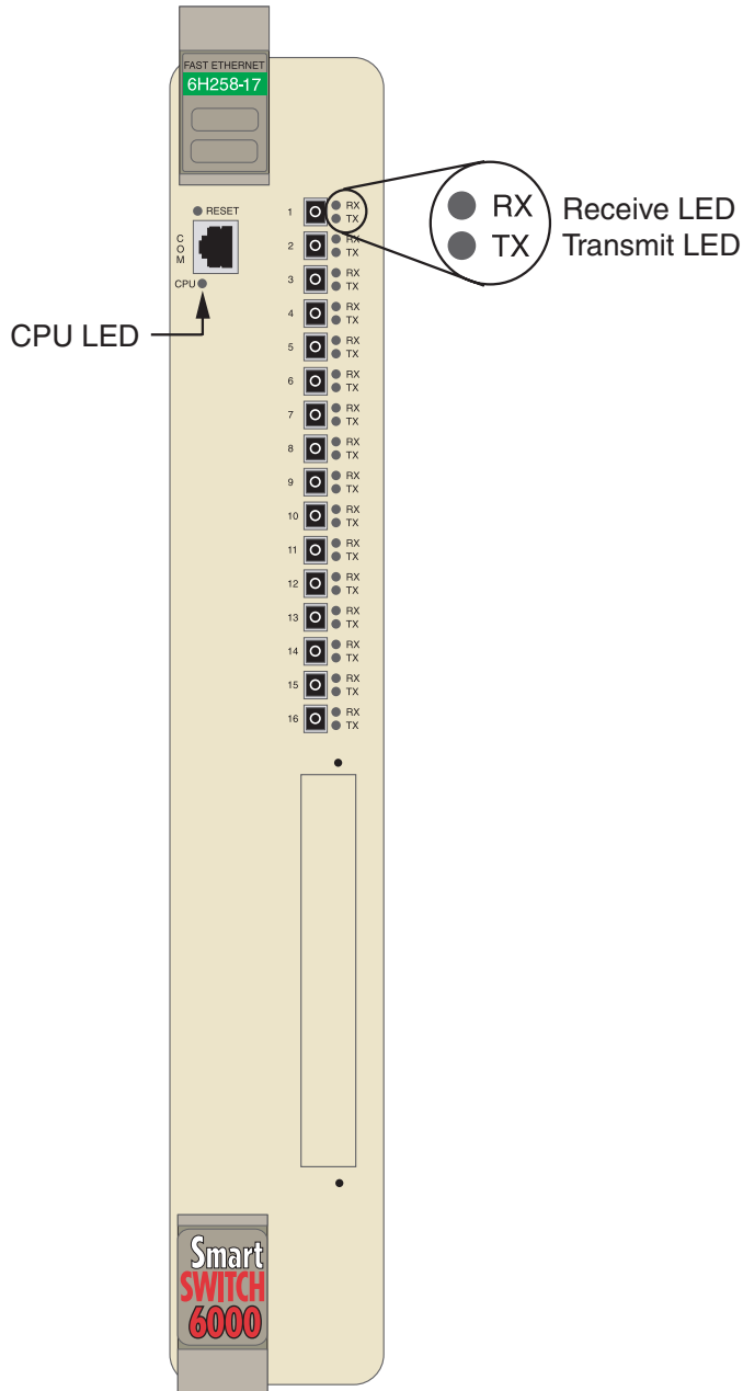
Figure 4-1 LANVIEW LEDs
