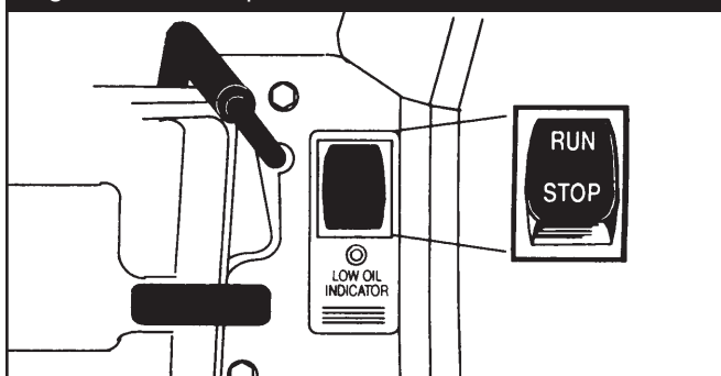
Figure 5 — Run/Stop Switch
