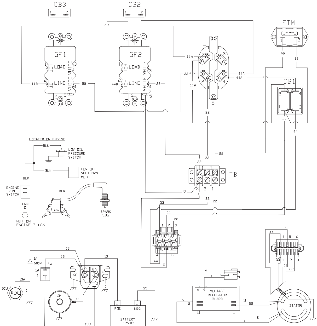
WIRE DIAGRAM
