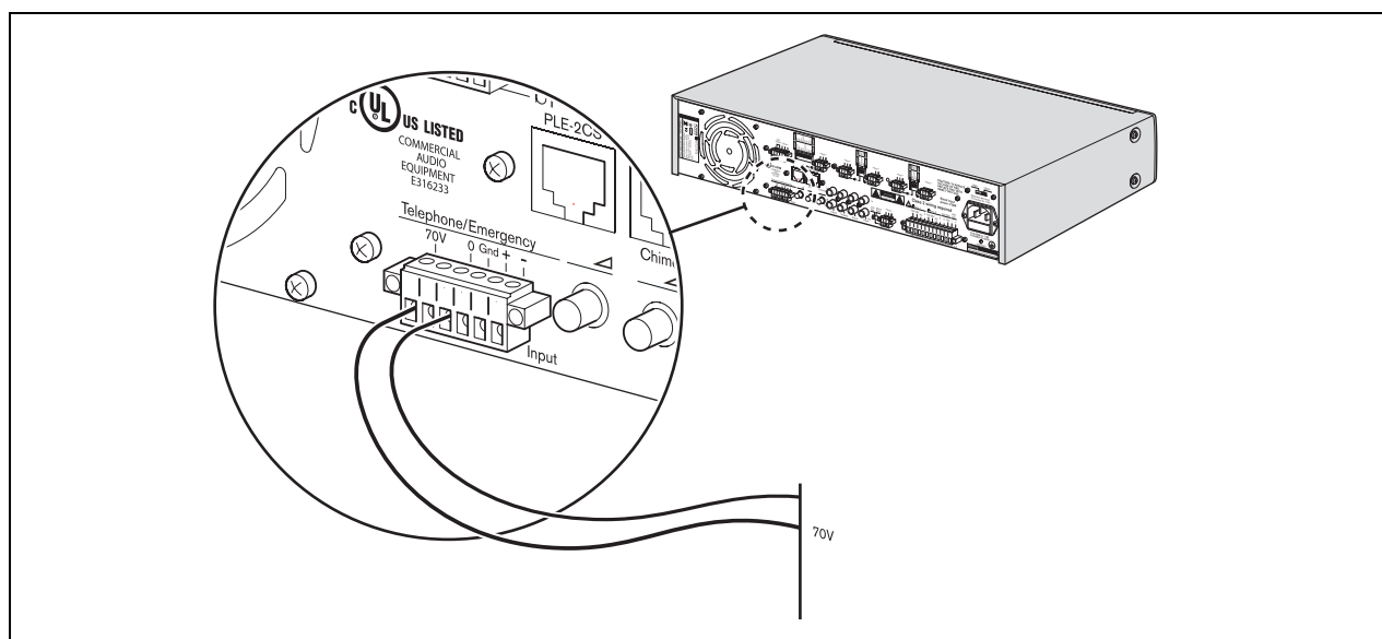
figure 4.4: Connecting 70 Volt input signal
