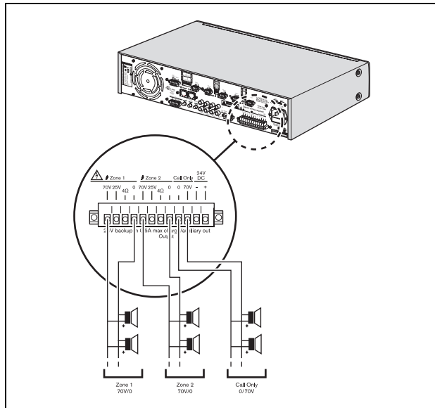
figure 4.8: Connecting speakers
