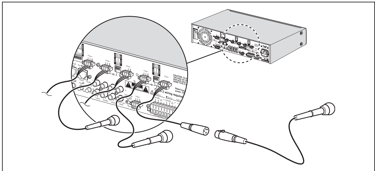
figure 4.3: Connecting microphone inputs
