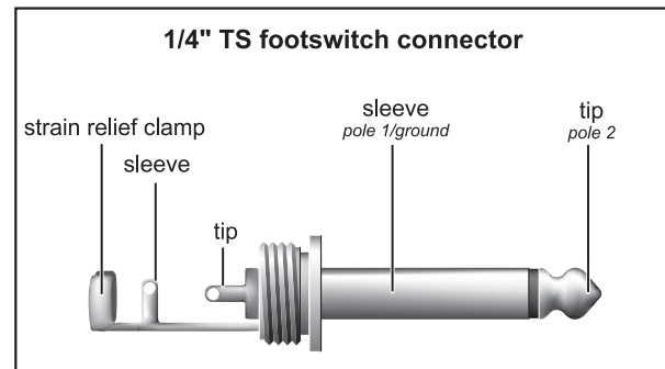
Fig. 4.2: 1/4" TS connector for the footswitch
