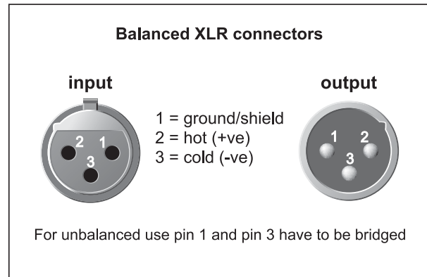
Fig. 4.1: XLR connections
