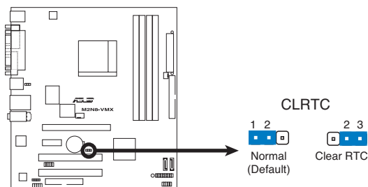
M2N8-VMX Clear RTC RAM
