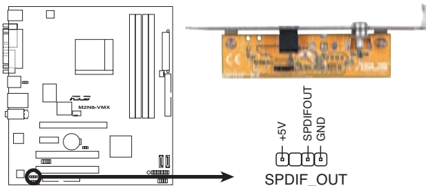
M2N8-VMX Digital Audio Connector
