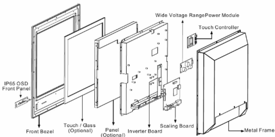
Figure 1.1 Basic Construction
