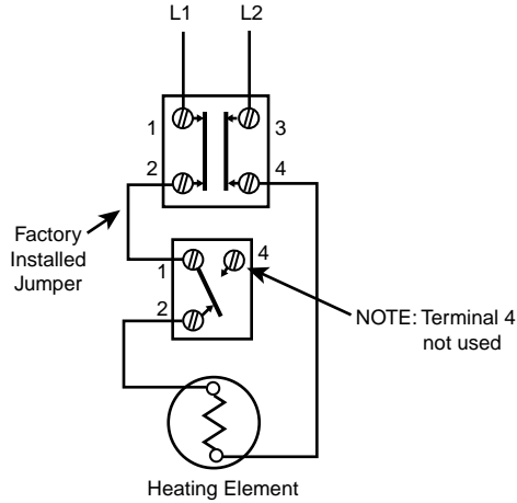
Single Element Circuit for Full Power Disconnect Through Both Power Conductors
