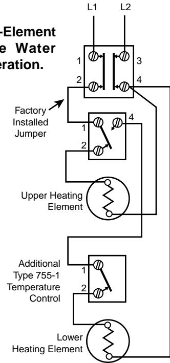
Double Element Limited Demand Circuit for Full Power Disconnect Through Both Power Conductors
