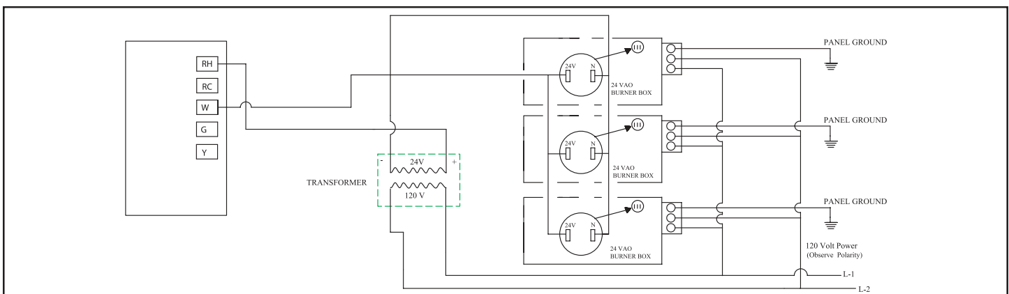
Single-stage heaters with a 1F77-51 thermostat. Multiple heaters, single thermostat. Picker Relays (relay boards) are installed.
