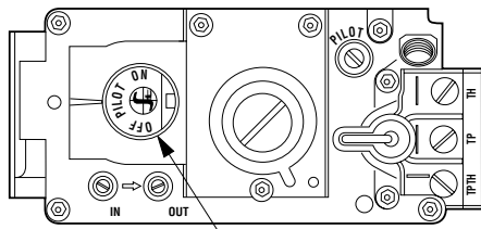
SIT Millivolt Valve Gas Control Knob
