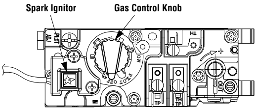
Honeywell Millivolt Valve
