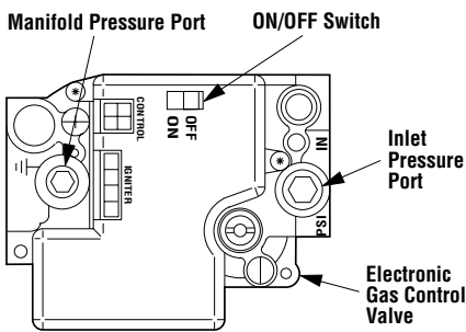
Honeywell Electronic Gas Valve
