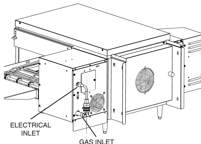
Figure 2-11. Junction Connection Box
