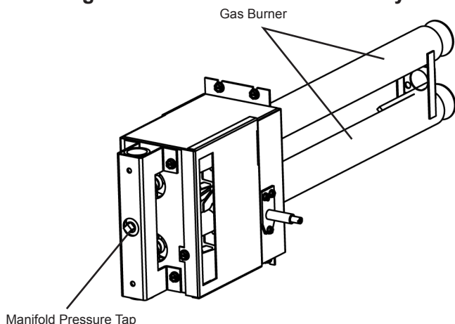
Figure 2-17. Burner Assembly
