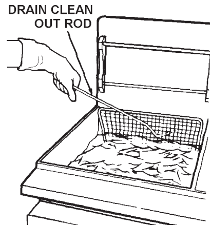
FIGURE 3. REMOVE SCREEN OVER TUBS/ELEMENTS
