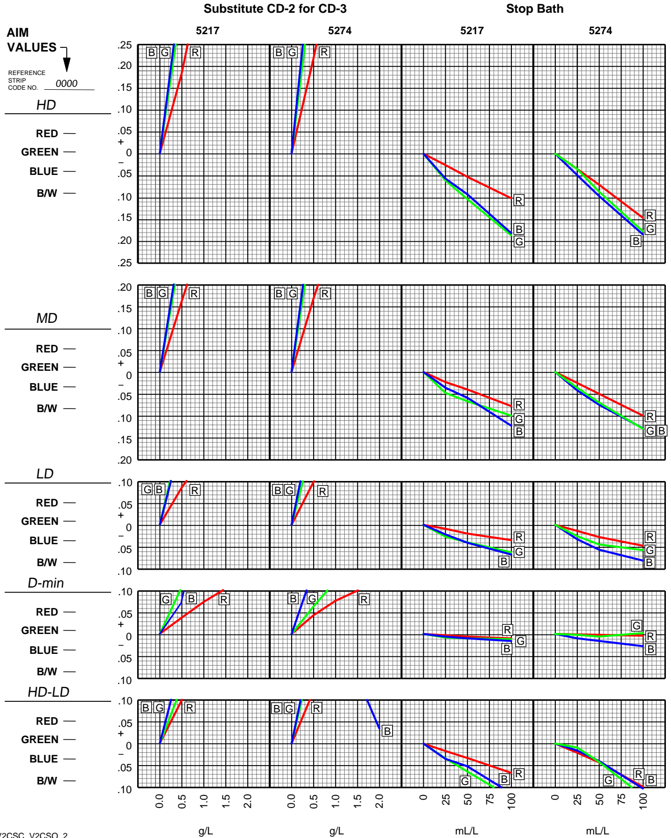
Figure 9 Effects of CD-2 for CD-3 and Stop Bath Contamination
