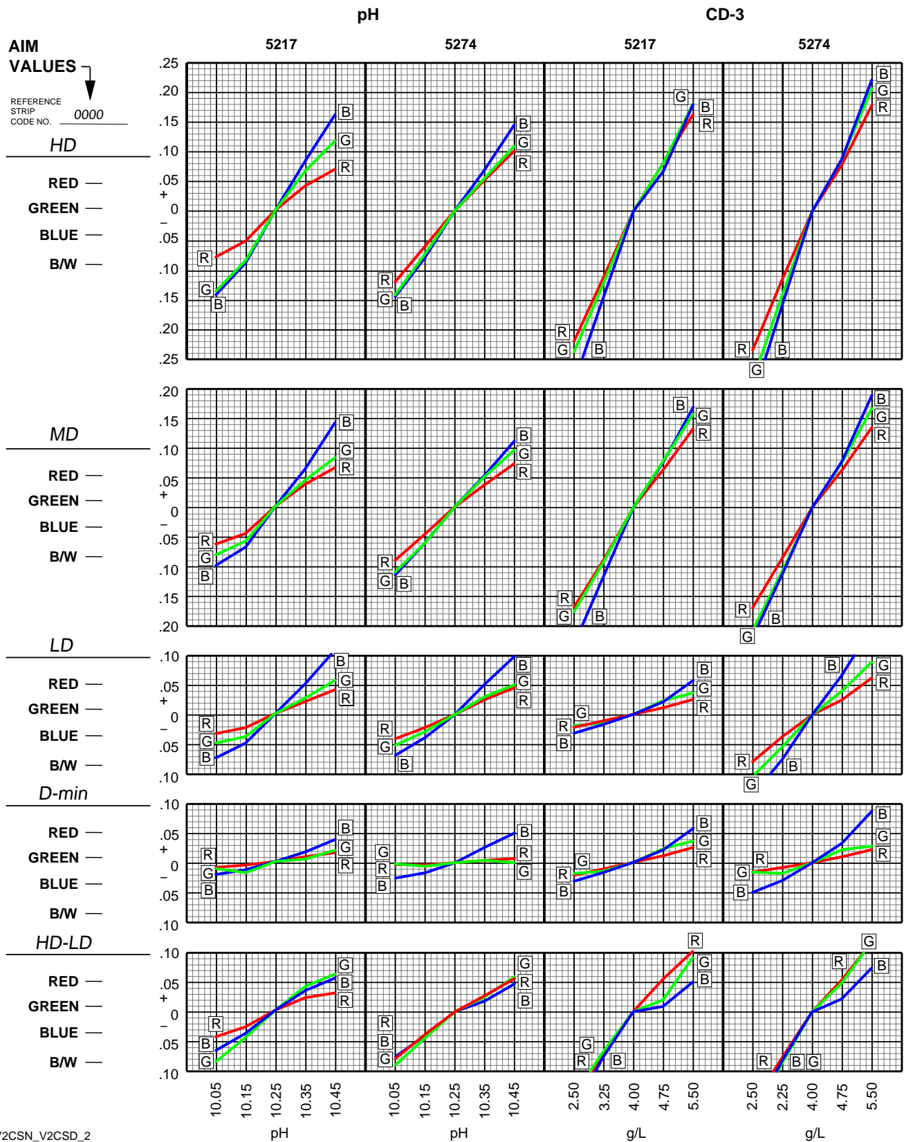
Figure 5 Effects of pH and CD-3 Variations
