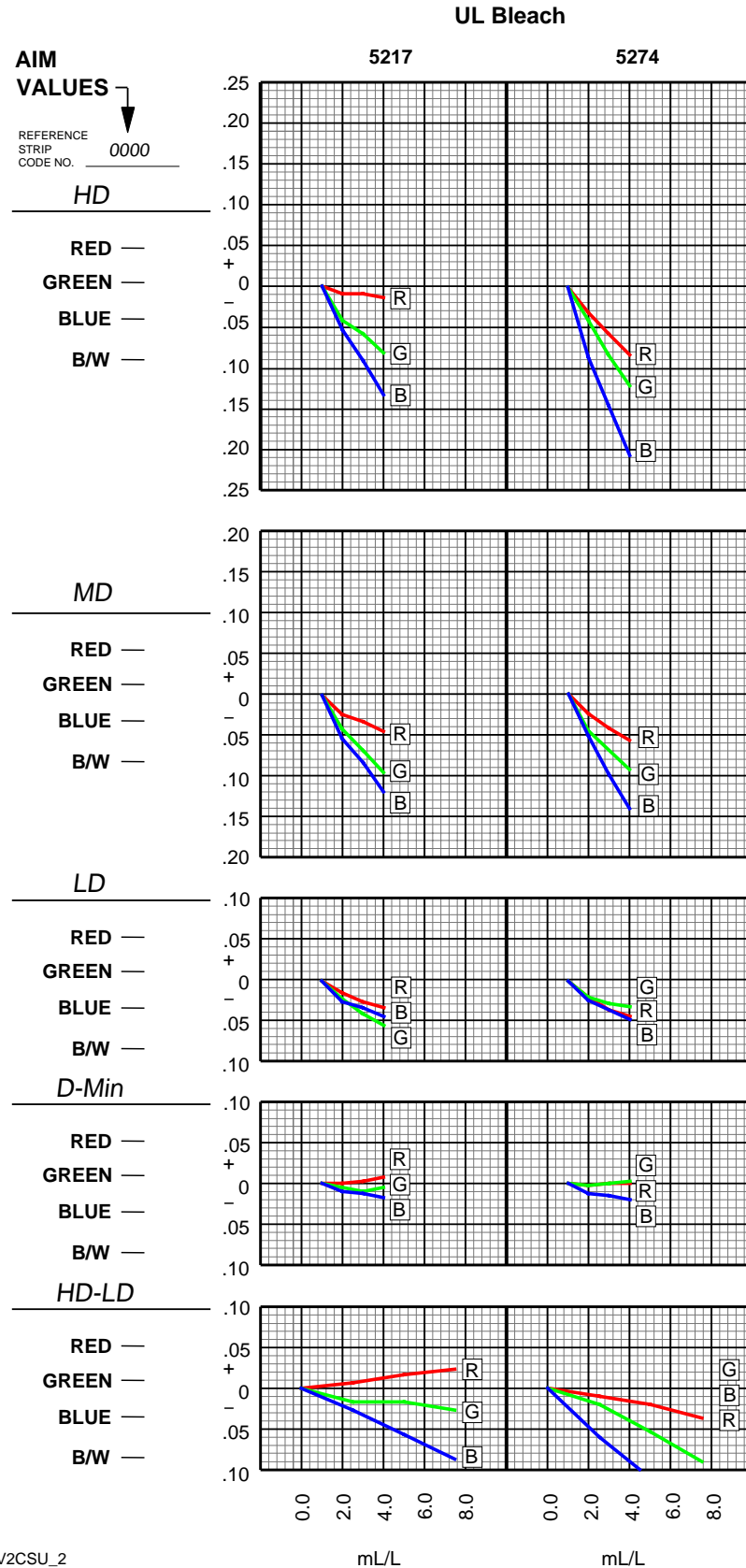
Figure 10 Effects of Bleach Contamination
