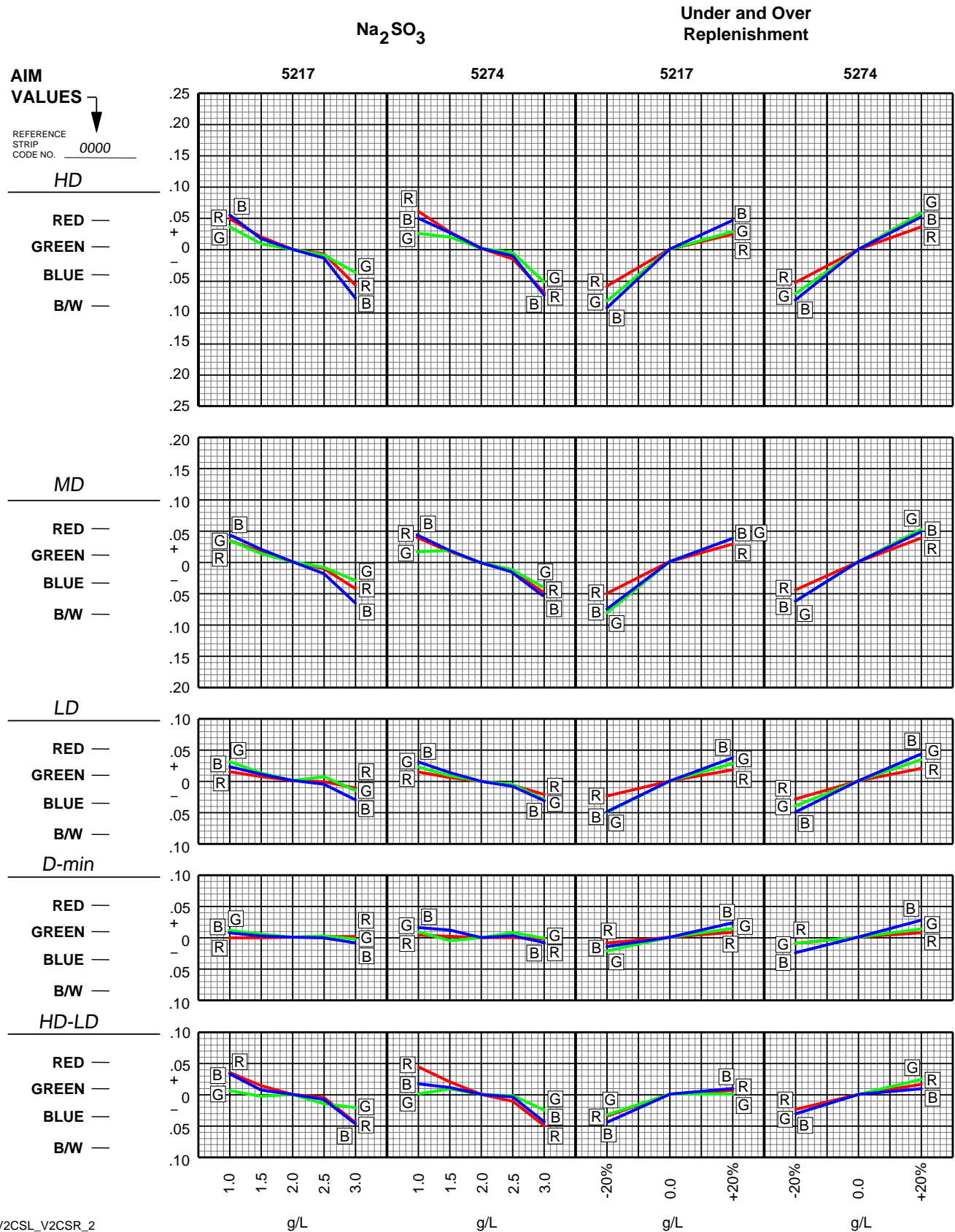
Figure 7 Effects of Na 2 SO 3 and Under and Over Replenishment Variations
