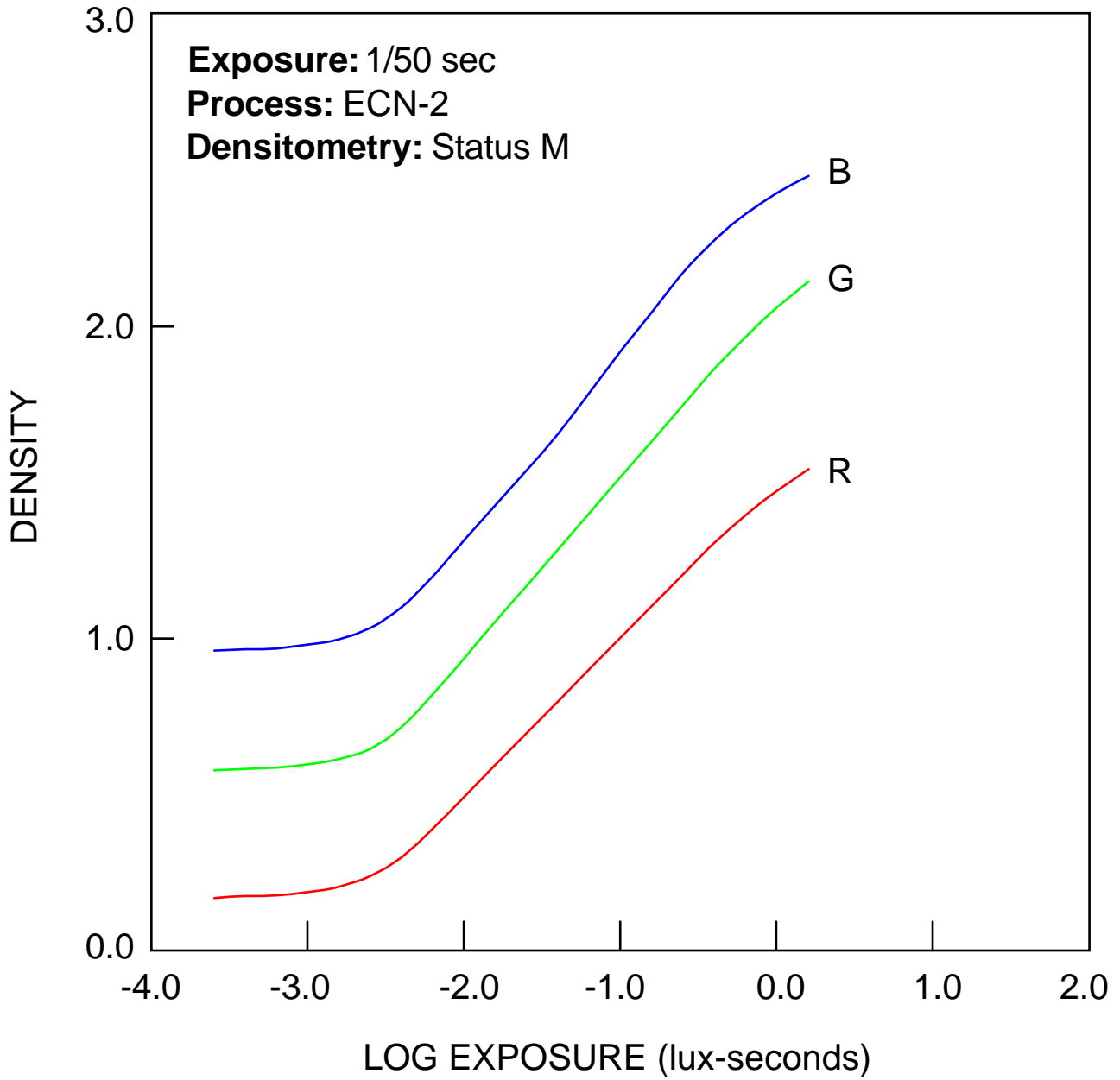
Figure 3 ECN-2 Control Strip Exposed on KODAK VISION2 200T Color Negative Film 5217
