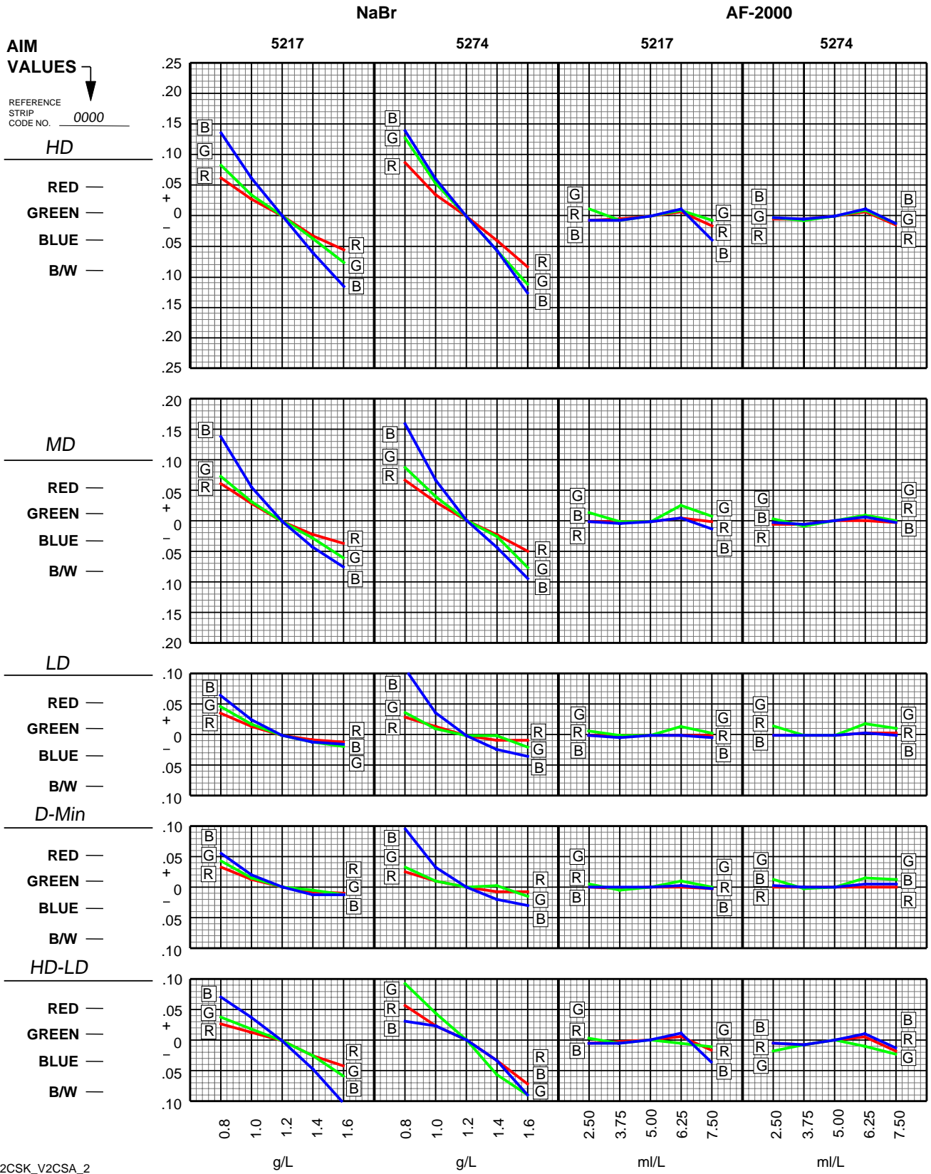
Figure 6 Effects of NaBr and AF-2000 Variations
