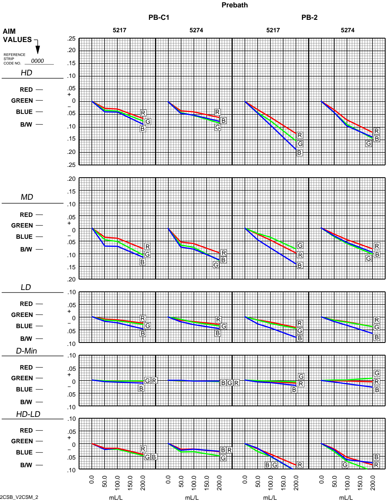
Figure 8 Effects of PB-C1 and PB-2 Prebath Contamination —VISION2 Control Strips versus VISION Control Strips in Process ECN-2 Developer
