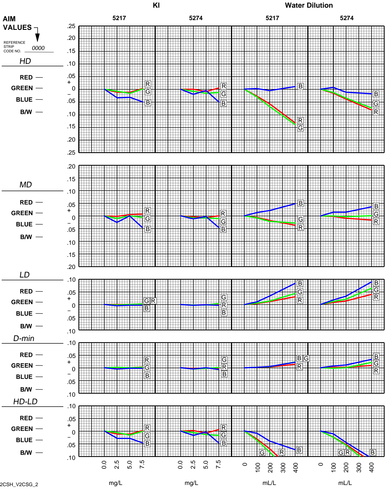
Figure 12 Effects of KI Contamination and Water Dilution —VISION2 Control Strips versus VISION Control Strips in Process ECN-2 Developer
