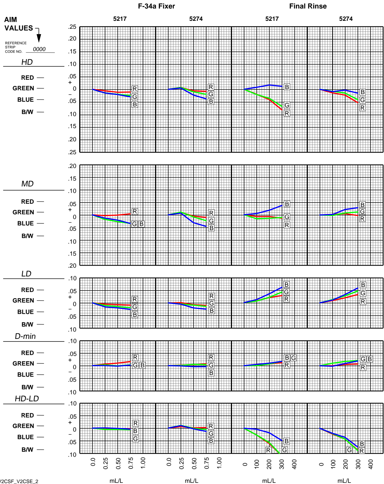
Figure 11 Effects of F-34a Fixer and Final Rinse Contamination —VISION2 Control Strips versus VISION Control Strips in Process ECN-2 Developer
