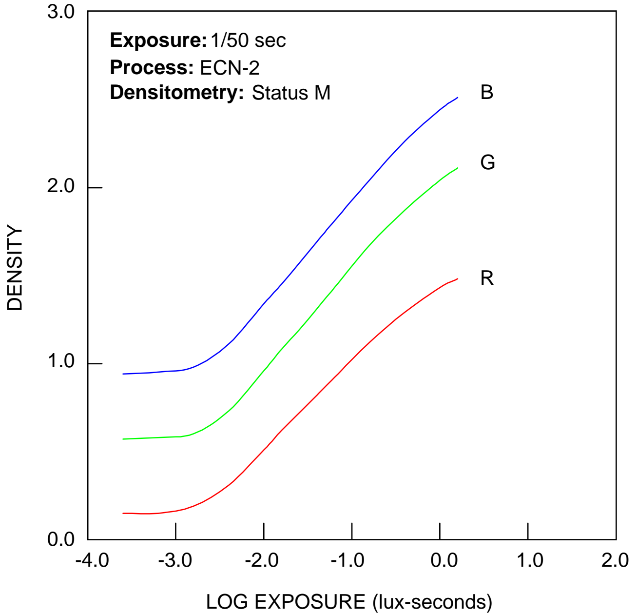
Figure 2 ECN-2 Control Strip Exposed on KODAK VISION 200T Color Negative Film 5274
