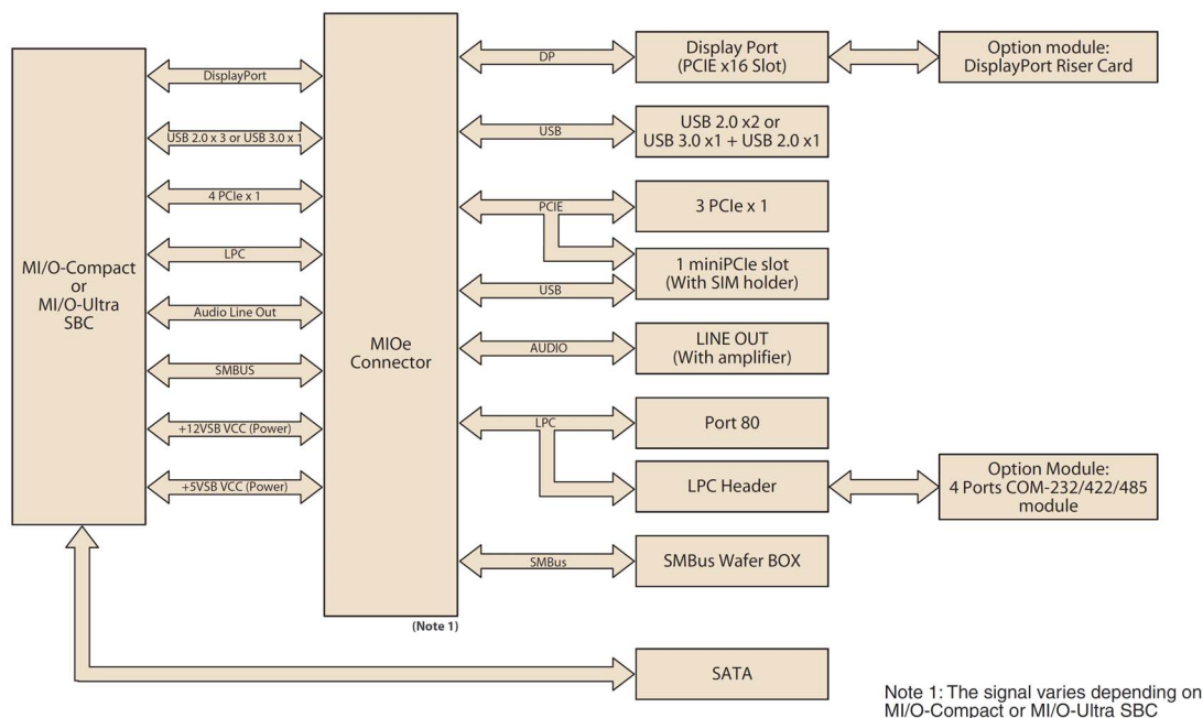
Figure 1.1 Block Diagram
